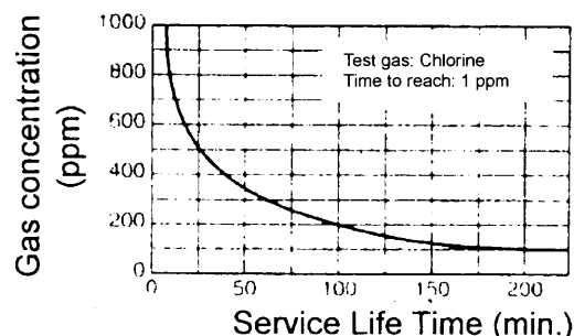
Breakthrough curve
